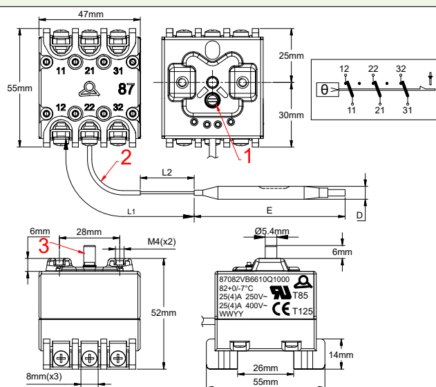
1. Sealing; 2. Sleeve; 3. Manual reset button
